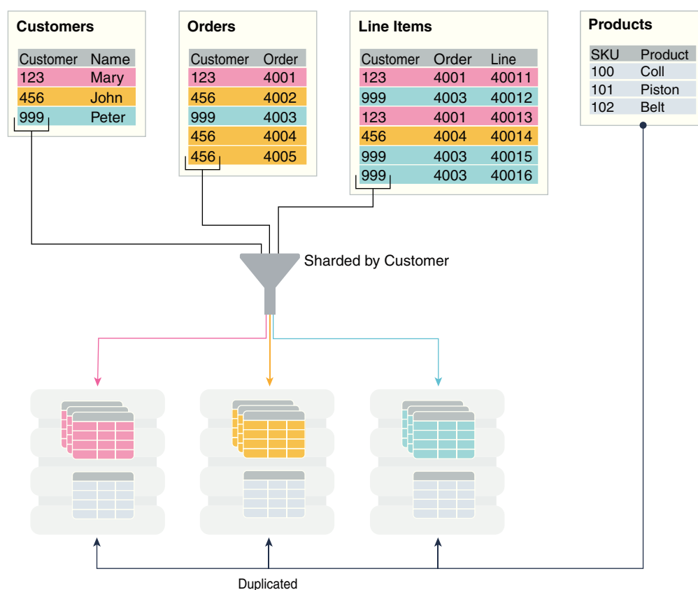
Figure 2-2 Sharded Tables and a Duplicated Table in an SDB
