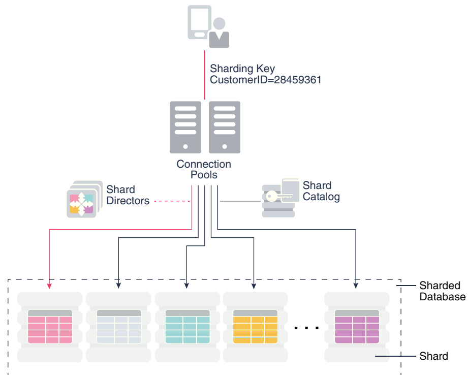
Figure 2-1 Oracle Sharding Architecture
