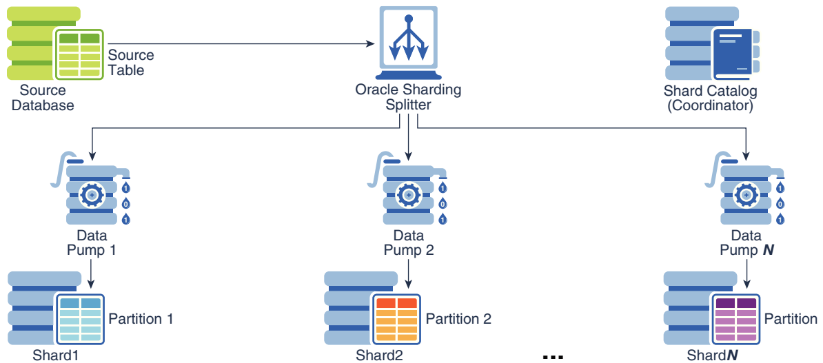
Figure 9-3 Loading Sharded Tables Directly to the Database Shards
