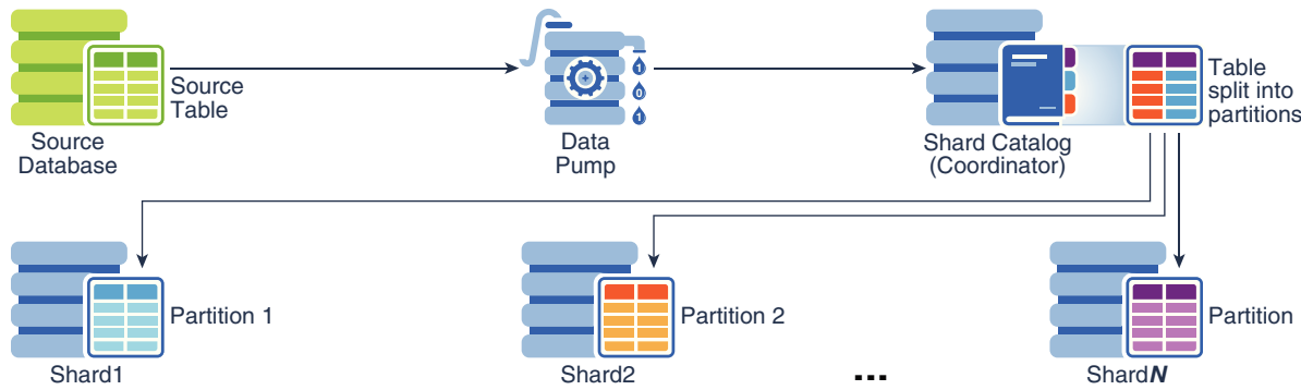
Figure 9-2 Loading Sharded Tables Using the Shard Catalog
