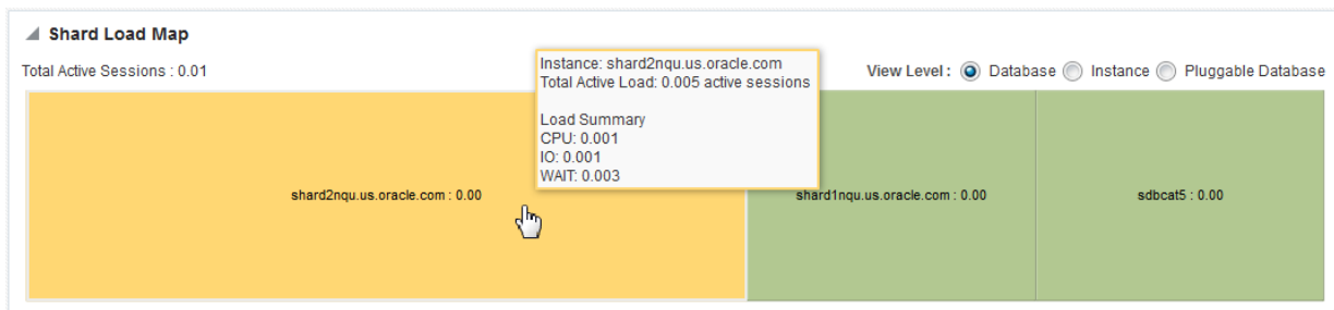
Figure 10-3 Sharded Database Shard Load Map
